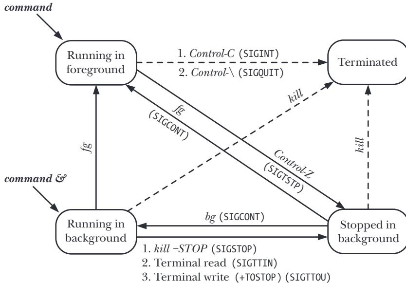
Figure 34-2: Job-control states
